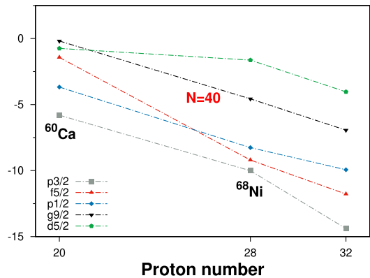
FIG. 5. Neutron effective single particle energies of the LNPS ^\dagger effective interaction.
